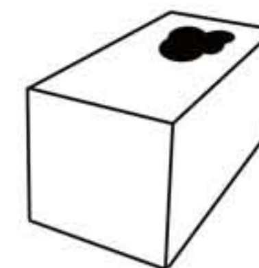
Meuble PLANT I XL en mm :: L 350 :: l 120 :: H 400 :: L 700 :: l 120 :: H 400 :: L 700 :: l 800 :: H 400
